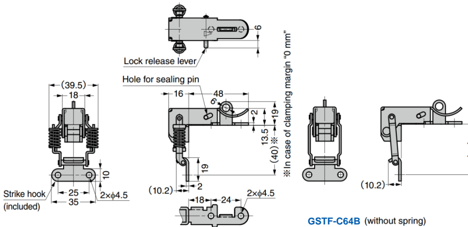
GSTF-C64A (with spring) Gasket is unnecessary.
